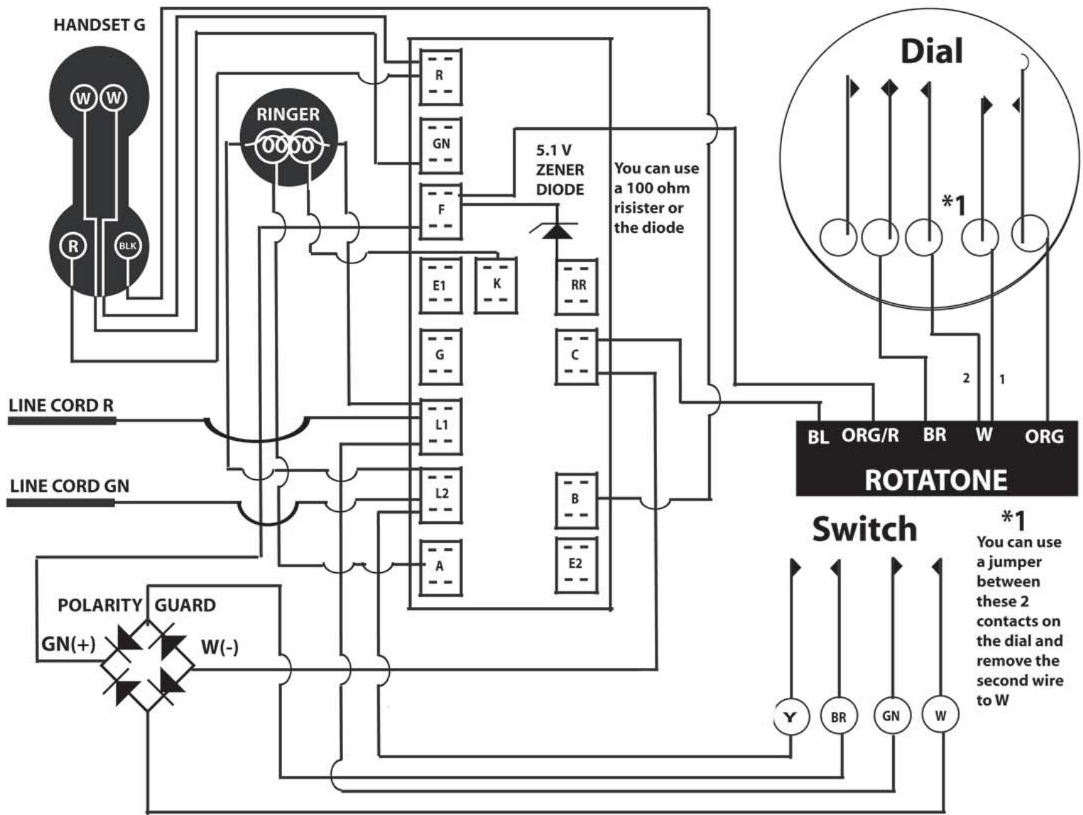
Rotatone with Western Electric 2500 Network and Automatic Electric Dial
